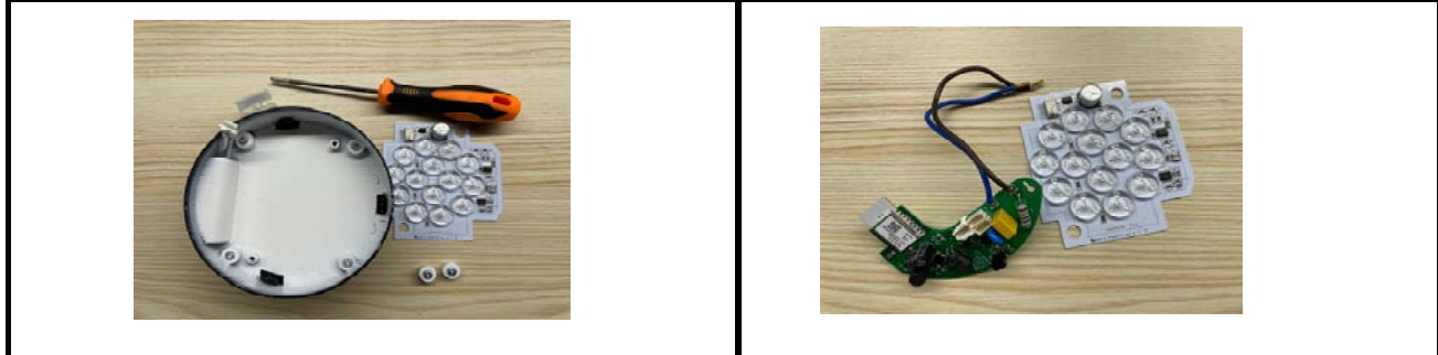
5. Unscrew and remove the LED board 6. Module 252VDC 27mA
