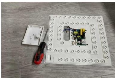
5. Unscrew and remove the protective shell of the control board
